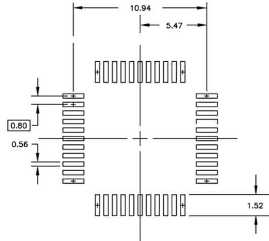
SUGGESTED PAD LAYOUT 44 PIN TQFP, 10*10*1.0
