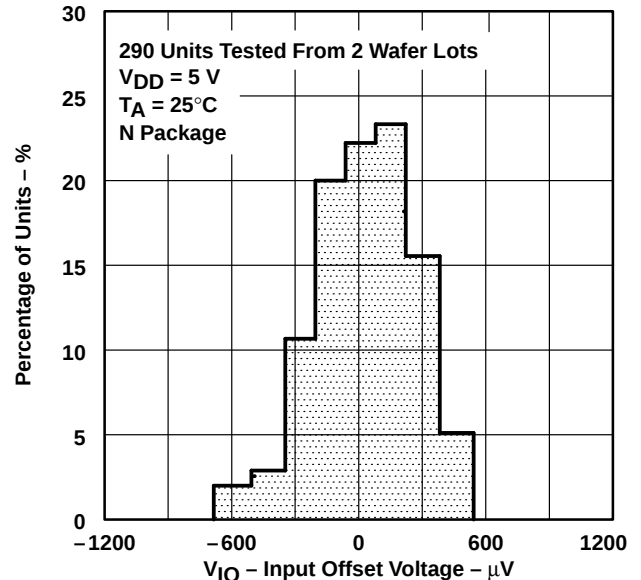
DISTRIBUTION OF TLC279 INPUT OFFSET VOLTAGE
