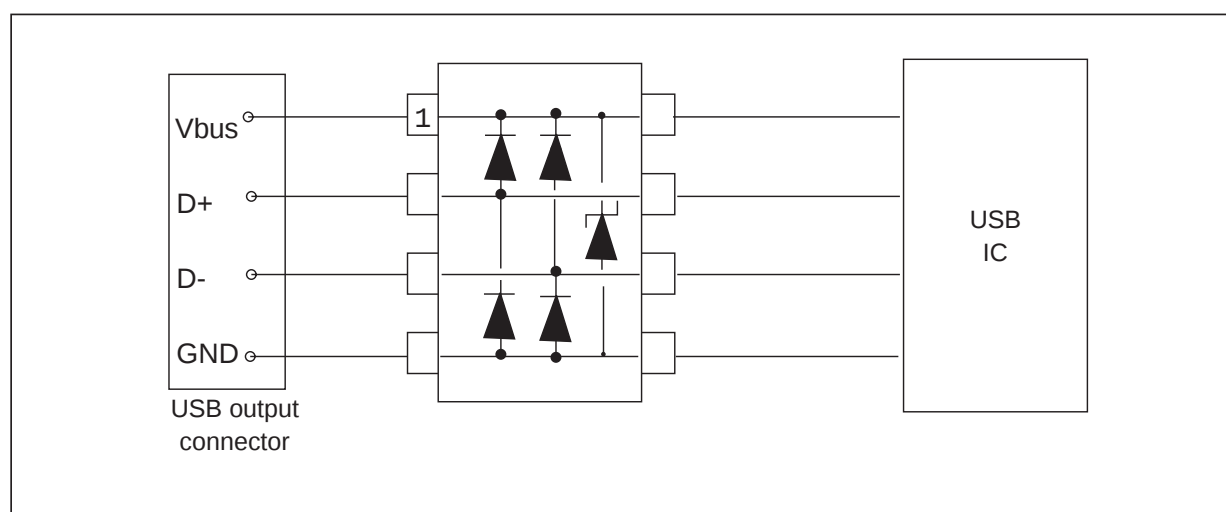
Fig. A3: recommended configuration for USB port protection.
